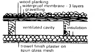
8 Cold roof - light construction
